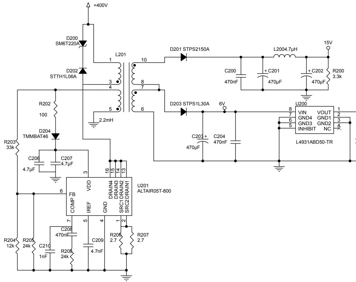
Figure 3. STEVAL-IPFC01P1 schematic - auxiliary power supply
