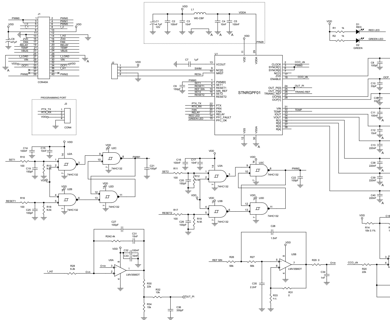
Figure 5. STEVAL-IPFC01C1 schematic
