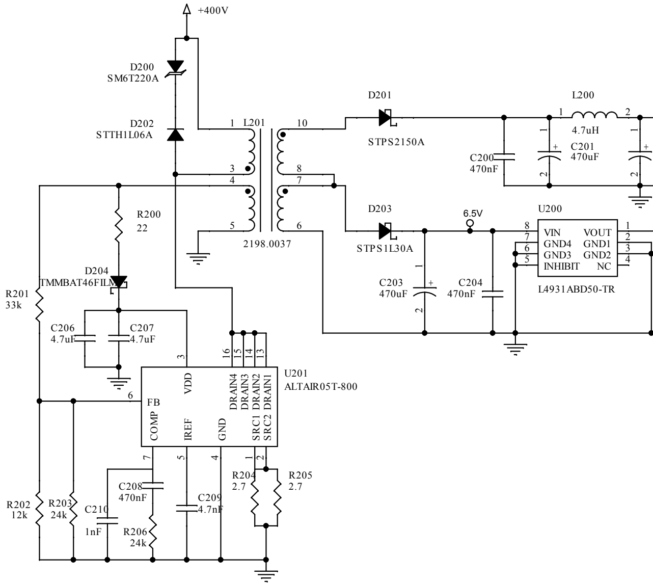
Figure 3. STEVAL-IPFC02P1 schematic - auxiliary power supply
