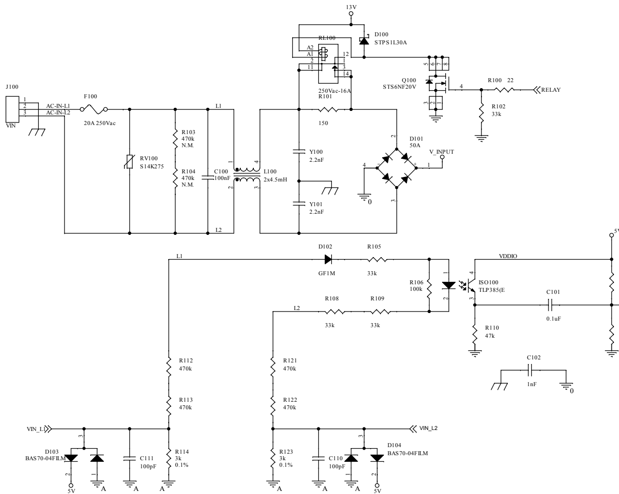
Figure 2. STEVAL-IPFC02P1 schematic - input section
