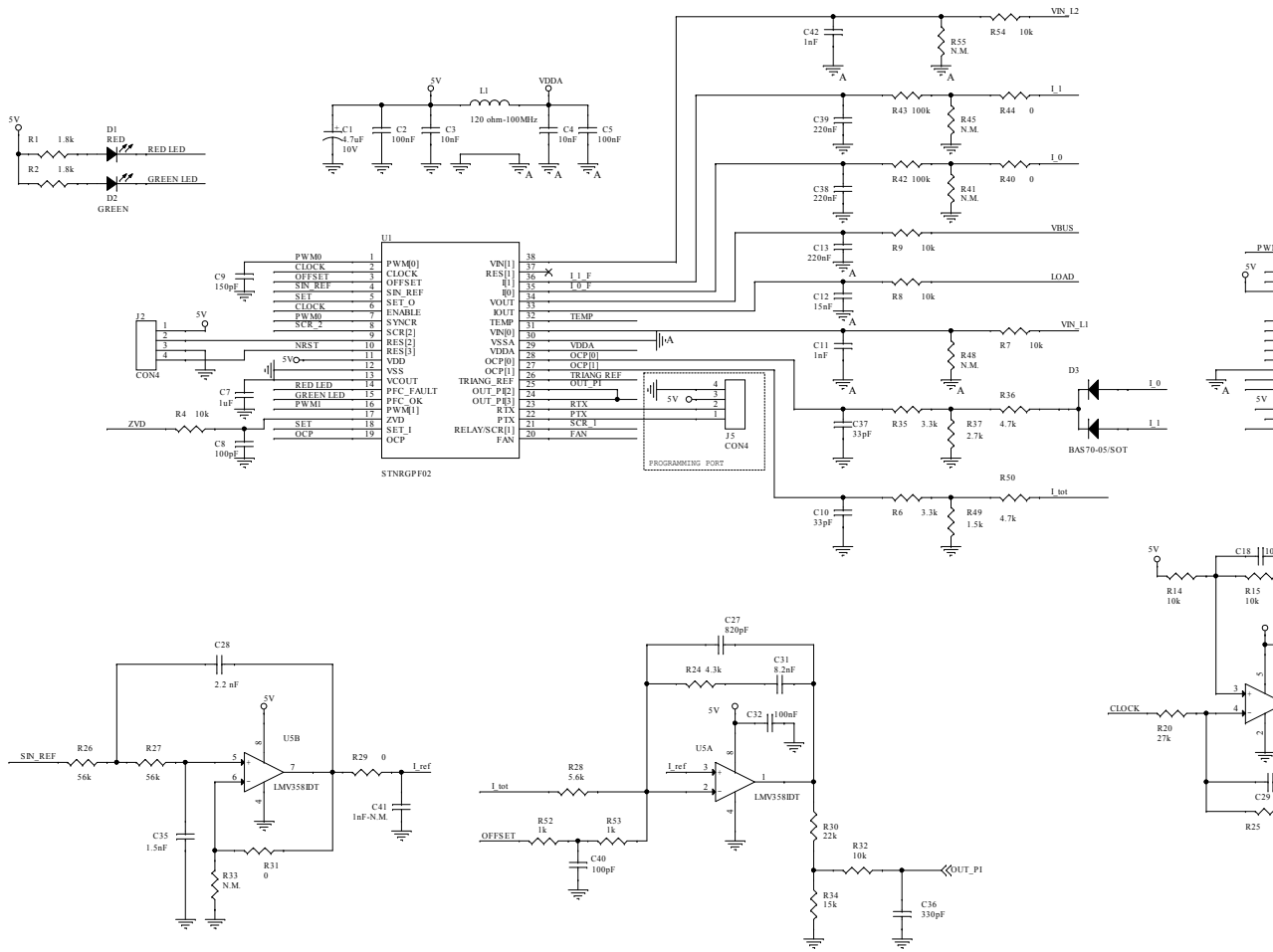
Figure 5. STEVAL-IPFC02C1 schematic
