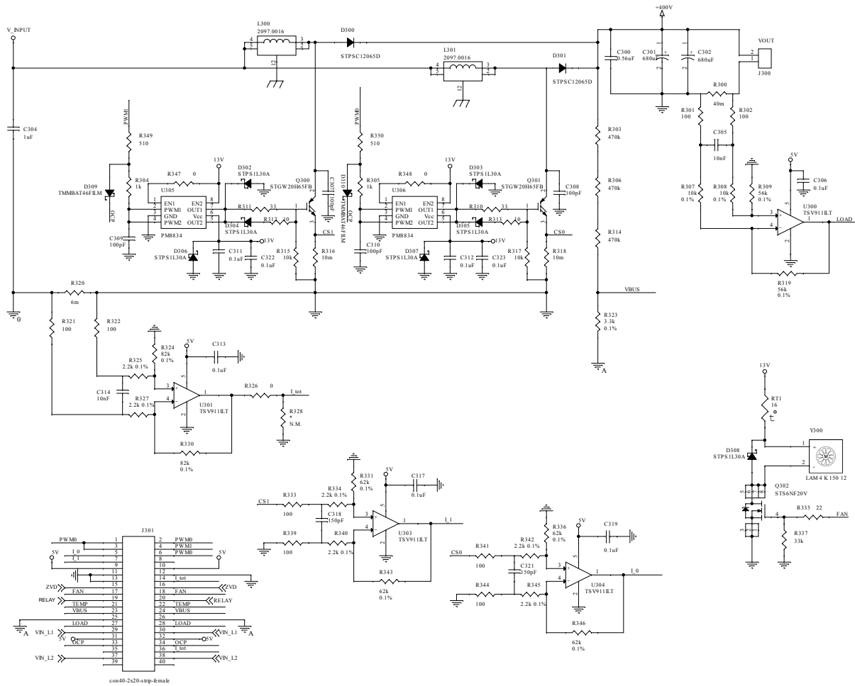
Figure 4. STEVAL-IPFC02P1 schematic - boost interleaving section
