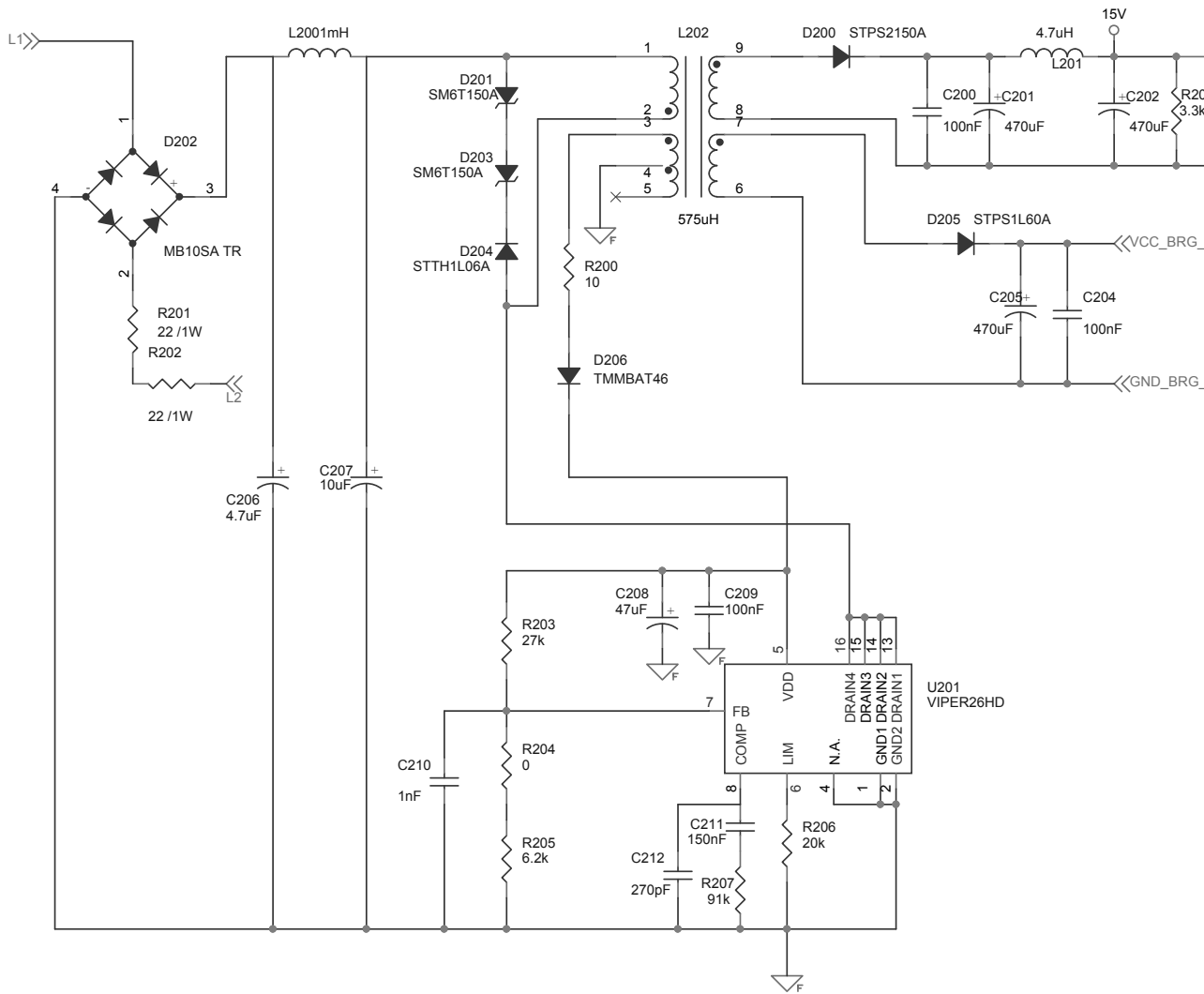
Figure 3. STEVAL-IPFC12P1 schematic - auxiliary power supply
