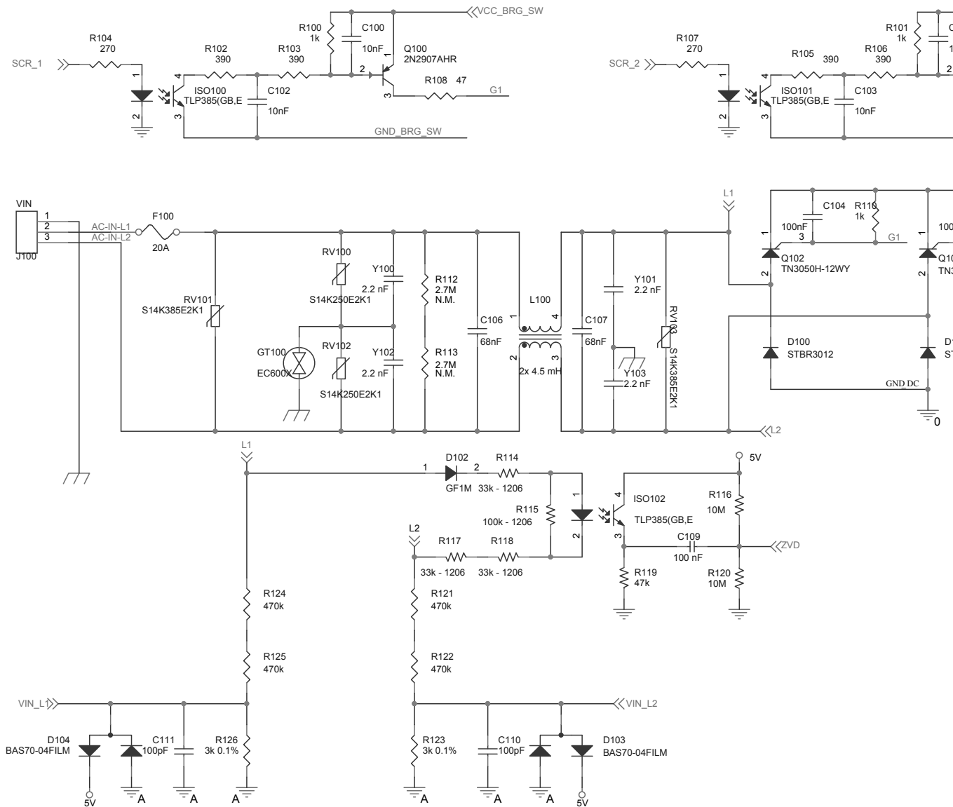
Figure 2. STEVAL-IPFC12P1 schematic - input section
