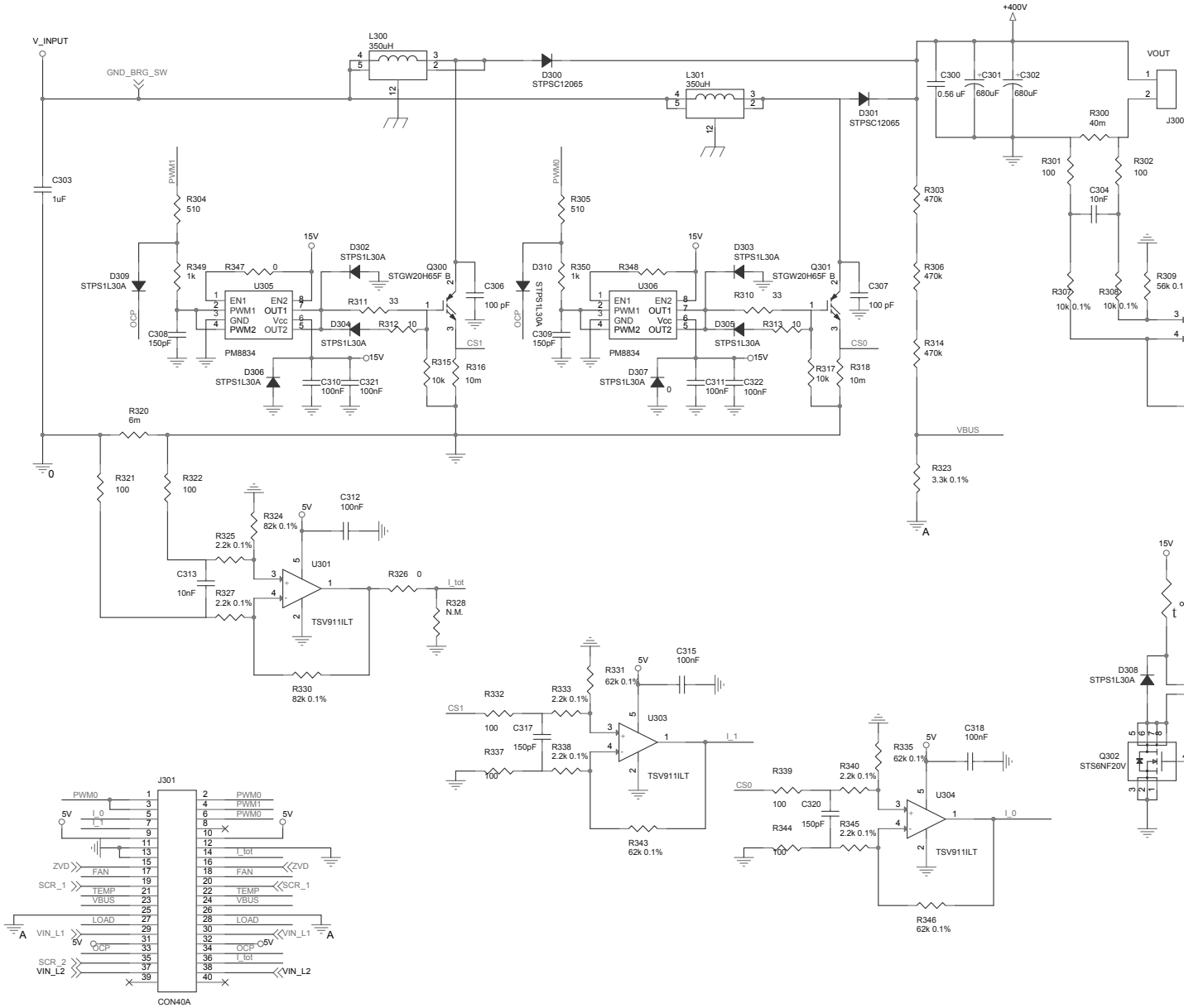
Figure 4. STEVAL-IPFC12P1 schematic - boost interleaving section
