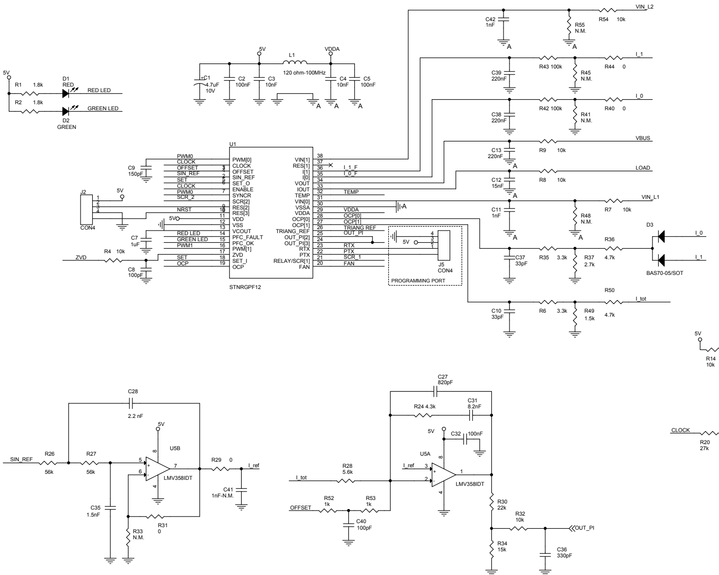
Figure 5. STEVAL-IPFC12C1 schematic
