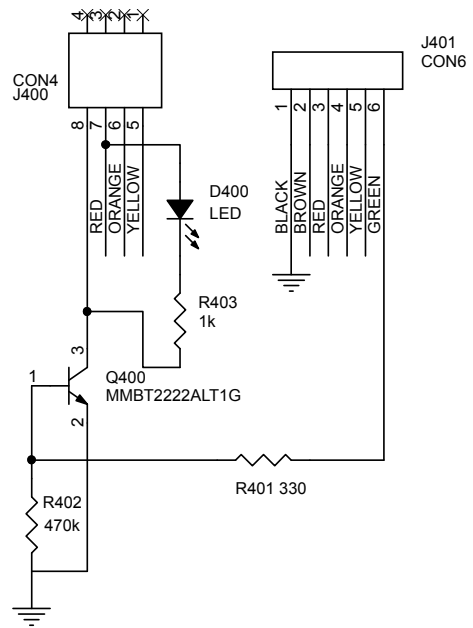
Figure 6. STEVAL-IPFC01A1 schematic
