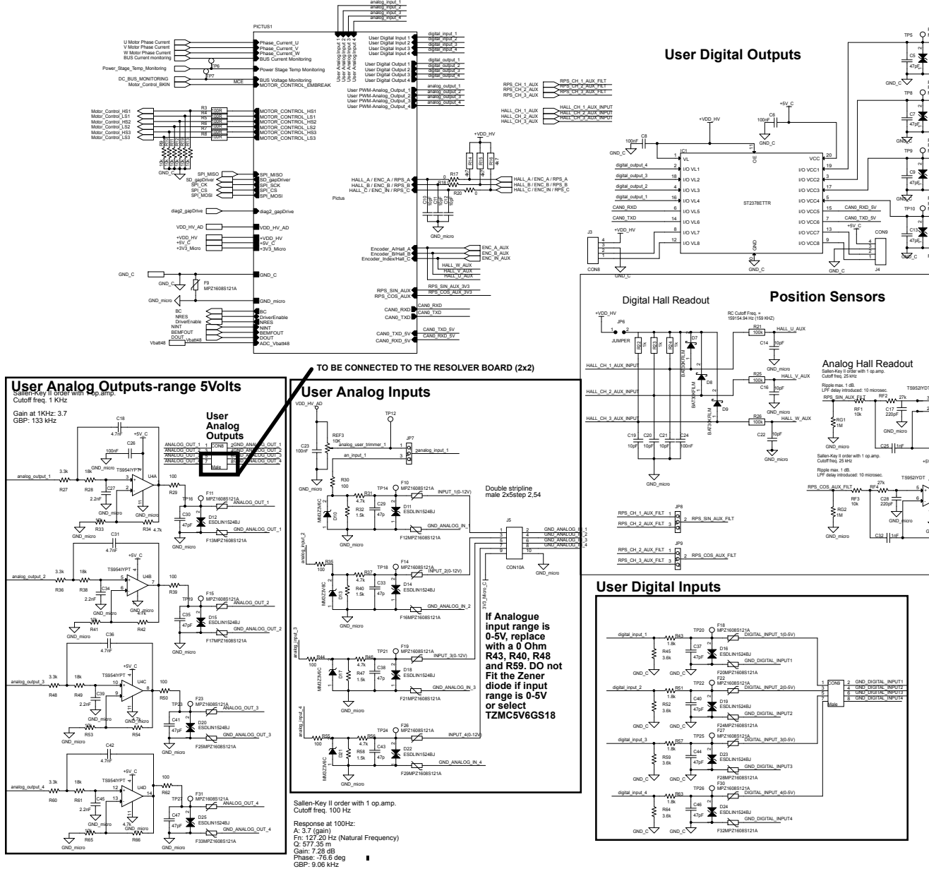
Figure 2. STEVAL-TTM002V1 control board - control stage
