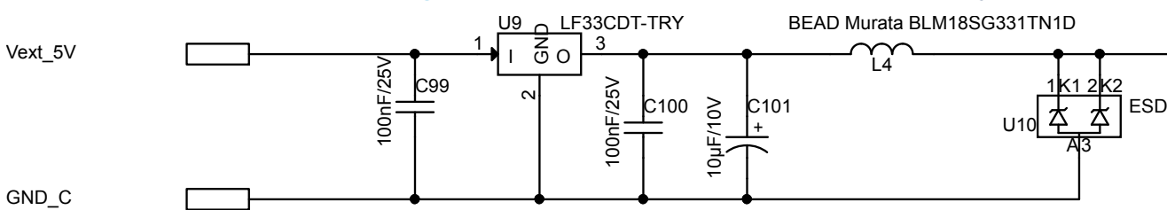
Figure 4. STEVAL-TTM002V1 control board - power supply block
