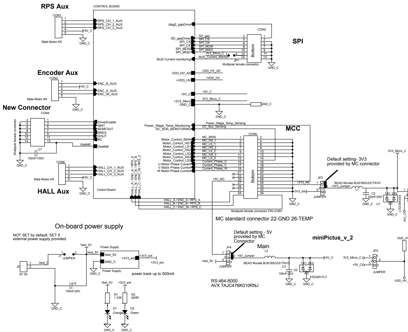
Figure 1. STEVAL-TTM002V1 control board - main block
