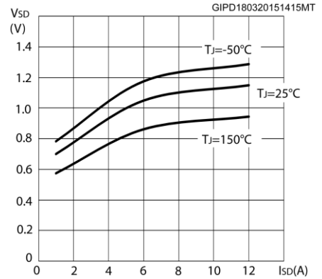
Figure 11: Source-drain diode forward characteristics
