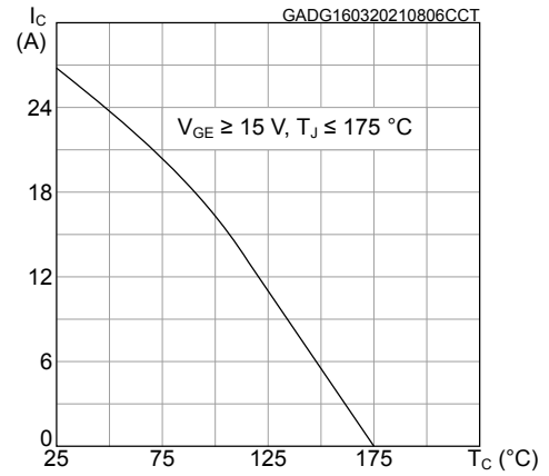
Figure 2. Collector current vs case temperature for TO-3PF
