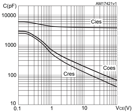
Figure 13. Capacitance variations
