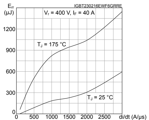
Figure 24. Reverse recovery energy vs diode current slope
