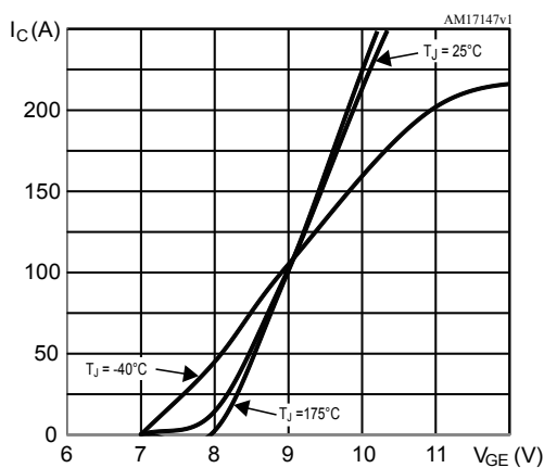
Figure 9. Transfer characteristics
