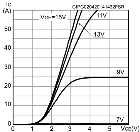
Figure 3. Output characteristics ( T_J = 25\text{ °C} )
