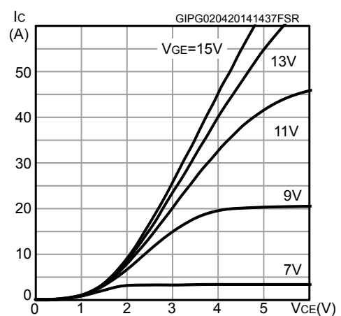
Figure 4. Output characteristics ( T_J = 175\text{ °C} )
