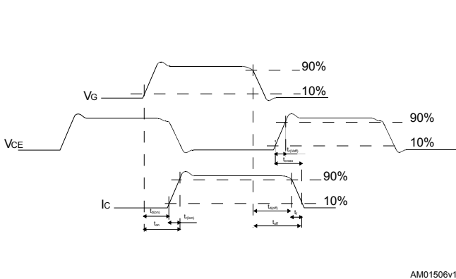
Figure 28. Switching waveform
