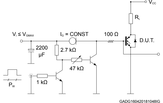
Figure 27. Gate charge test circuit
