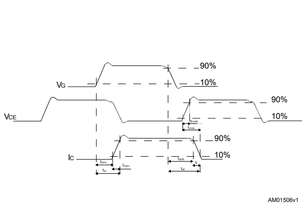
Figure 29. Switching waveform
