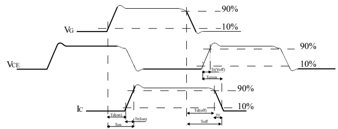
Figure 24. Switching waveform
