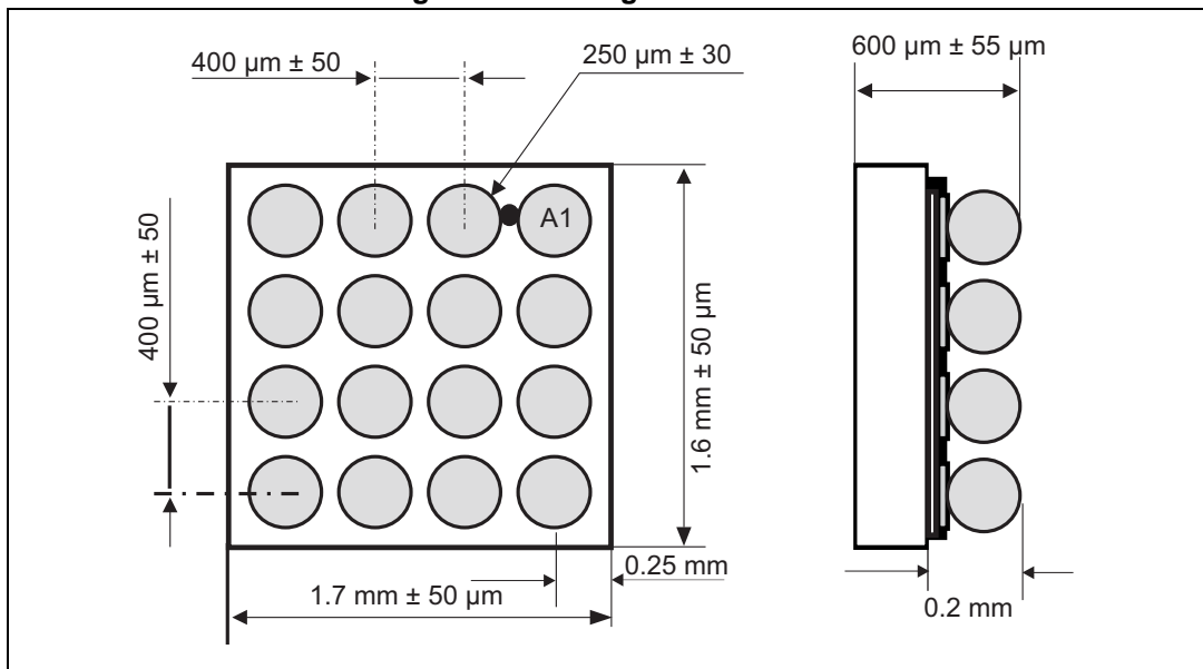
Figure 16. Package dimensions
