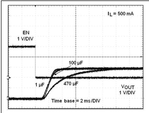
Figure 32. Voltage output turn-on delay time (STMP2161/2171, 3 V)
