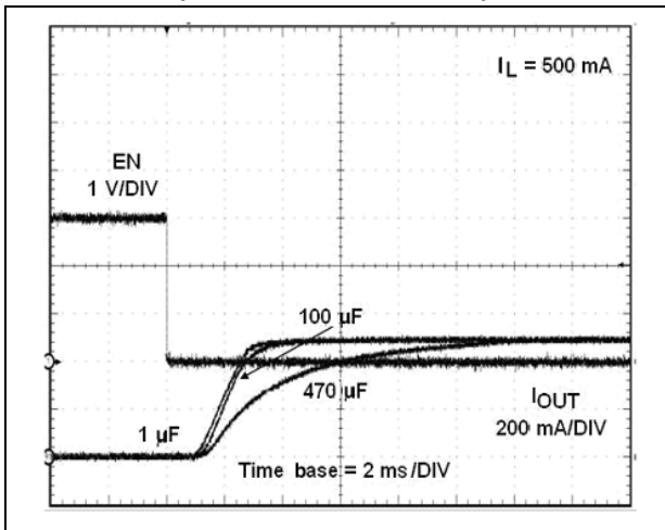
Figure 9. Current output turn-on delay time (STMP2141/2151, 3 V)
