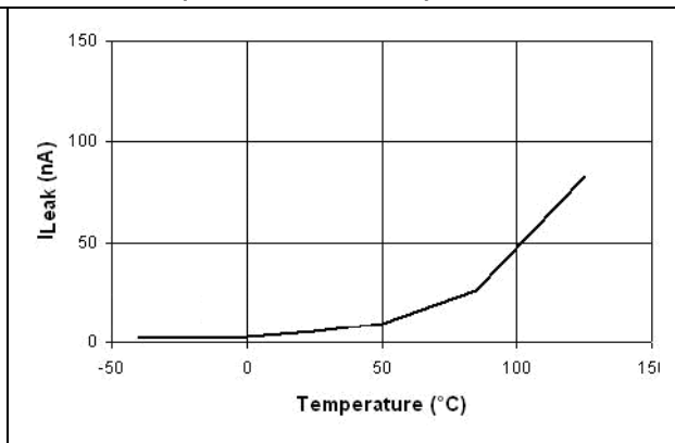
Figure 49. Switch leakage vs. temperature (STMPS2161/2171)
