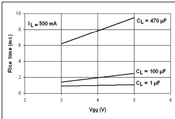
Figure 25. Output rise time vs. V_{IN} (STMPS2141/2151)
