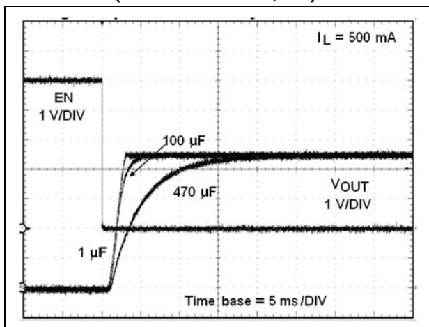
Figure 5. Current output turn-on delay time (STMPS2141/2151, 5 V)
