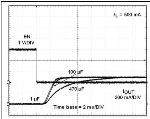
Figure 34. Current output turn-on delay time (STMP2161/2171, 3 V)
