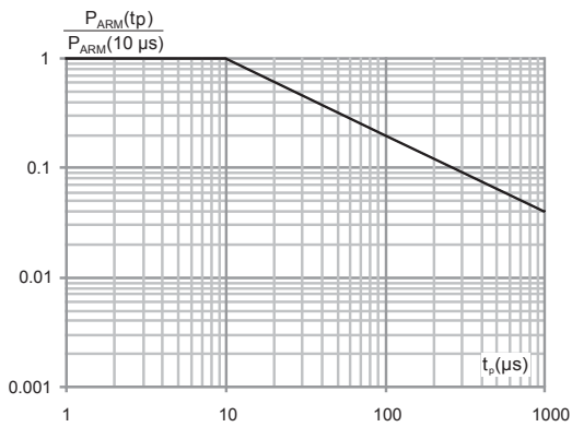
Figure 3. Normalized avalanche power derating versus junction temperature ( T_j = 125\text{ }^\circ\text{C} )
