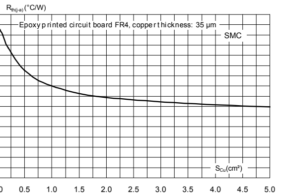
Figure 12. Thermal resistance junction to ambient versus copper surface under each lead (SMC)
