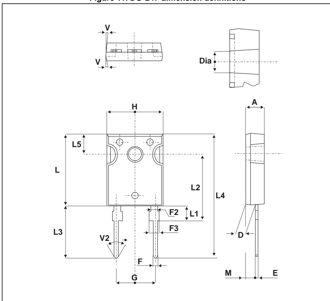
Figure 11. DO-247 dimension definitions
