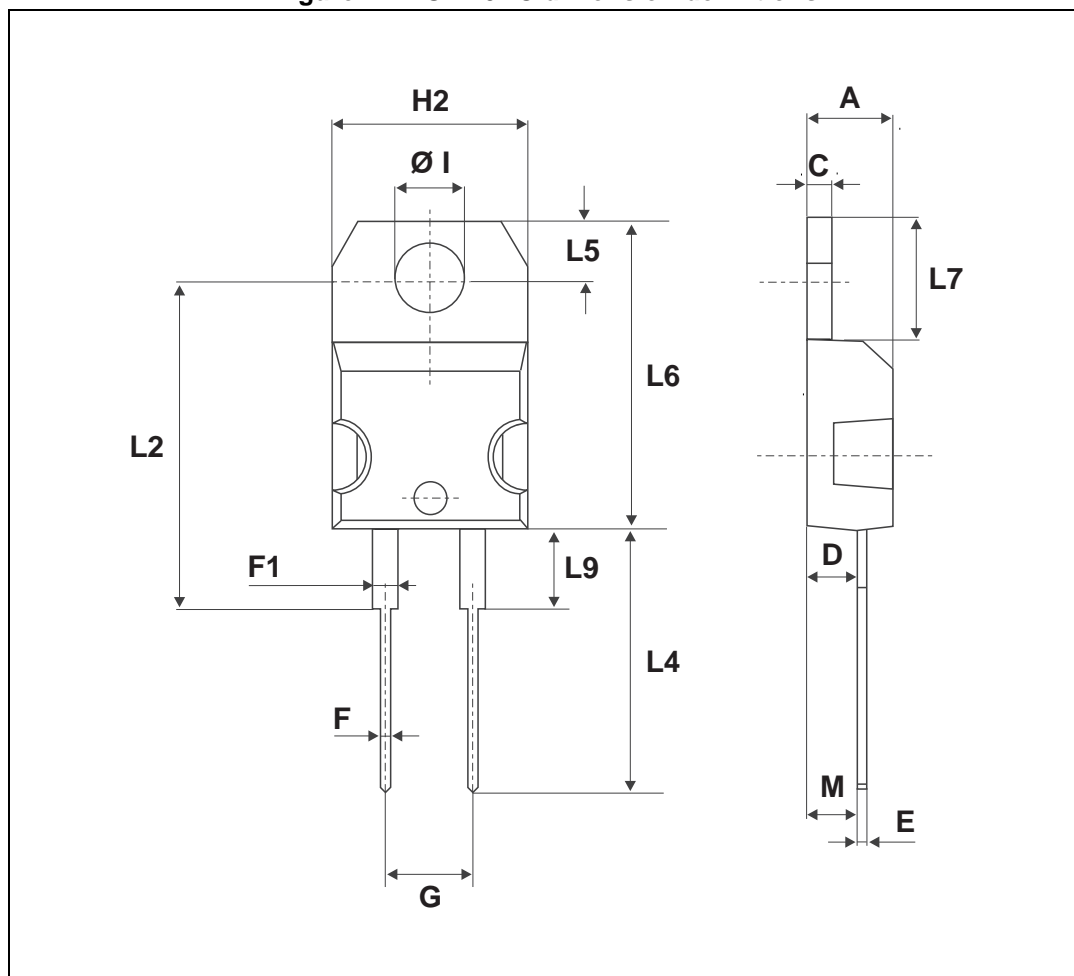
Figure 12. TO-220AC dimension definitions
