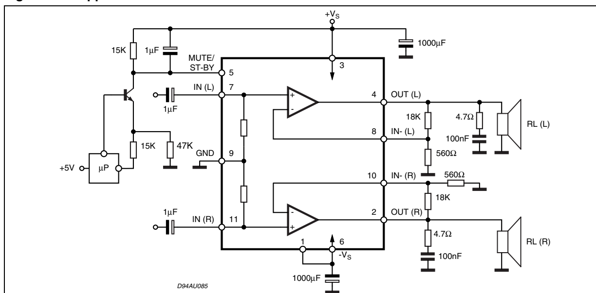
Figure 1. Applications circuit
