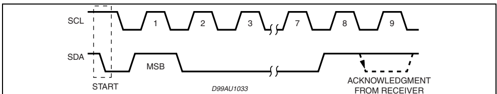
Figure 18. Acknowledge on the I 2 C BUS
