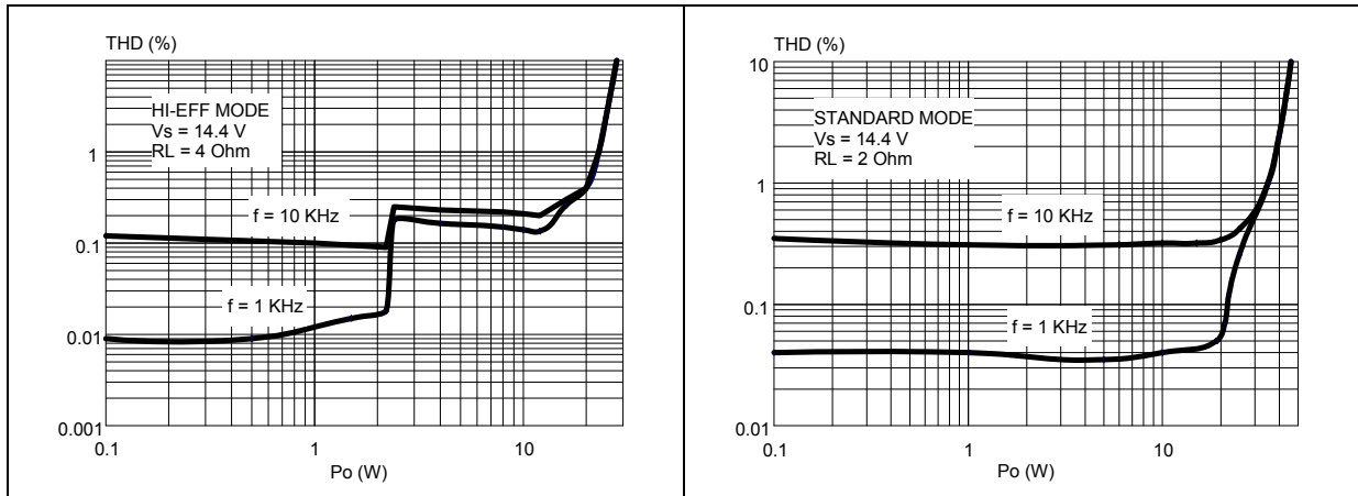
Figure 11. Distortion vs. frequency (4 Ω)
