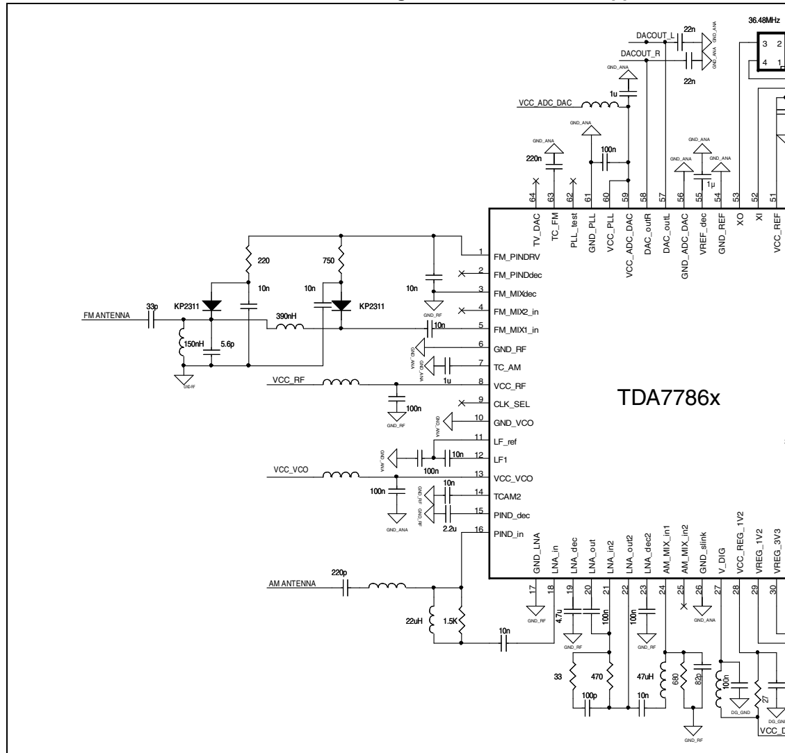
Figure 24. FM wide-band application
