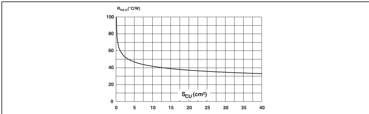
Figure 9. Junction to ambient thermal resistance versus copper surface under tab, PCB FR4, copper thickness 35\mu\text{m}
