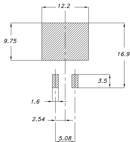
Figure 14. D 2 PAK recommended footprint (dimensions are in mm)
