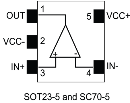
Figure 1. Pin configuration
