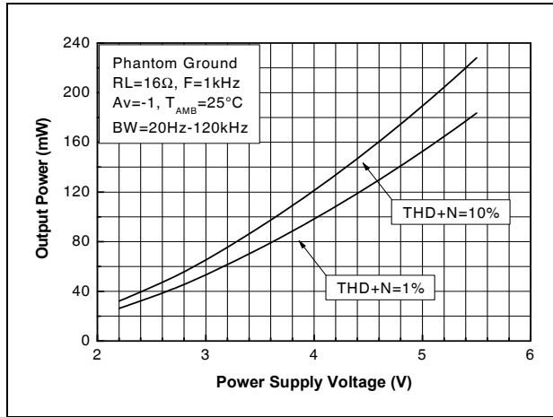
Figure 32. Output power vs. power supply voltage, PHG, R_L = 16 \Omega , F = 1 \text{ kHz}
