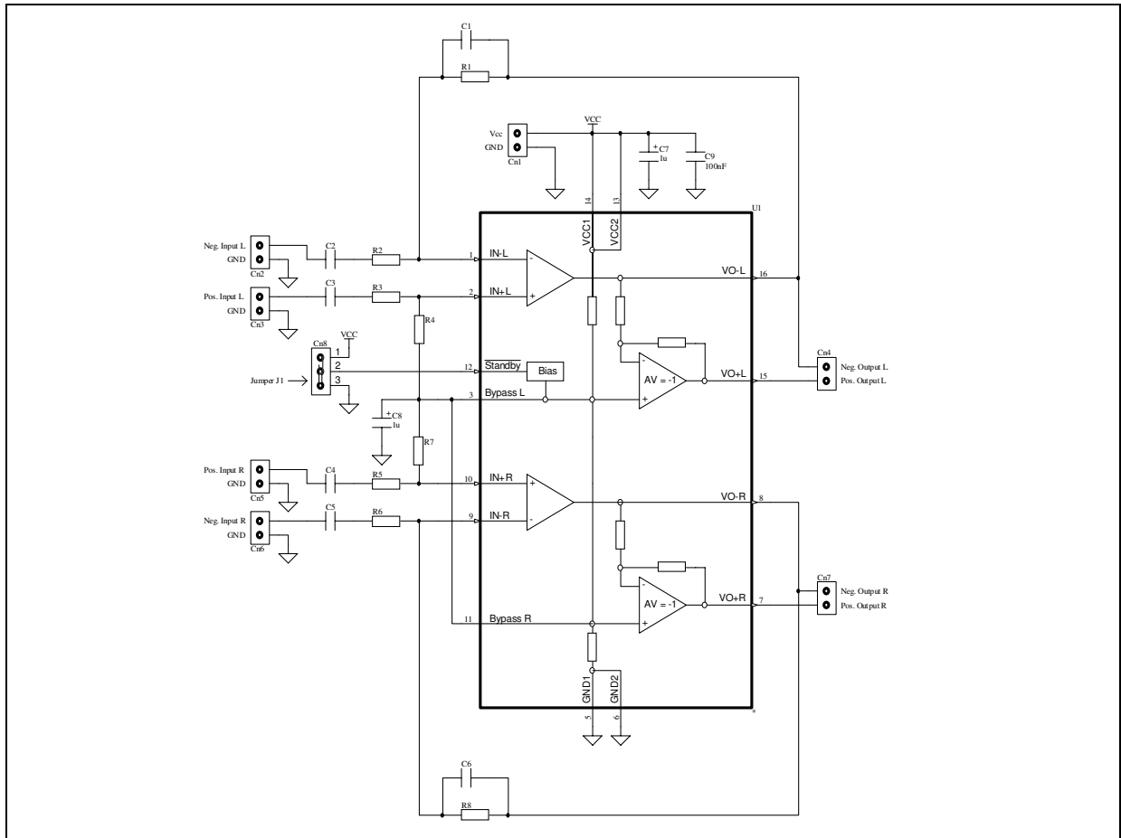
Figure 70: Demoboard schematic
