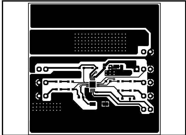
Figure 72: Top layer
