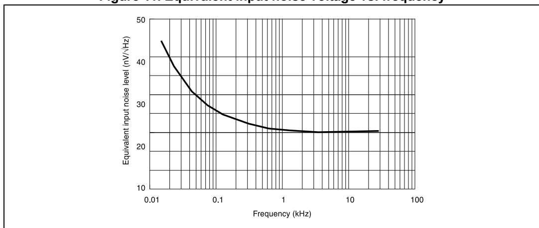
Figure 11. Equivalent input noise voltage vs. frequency
