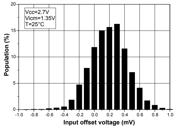
Figure 3. Input offset voltage distribution at V_{CC} = 2.7\text{ V}
