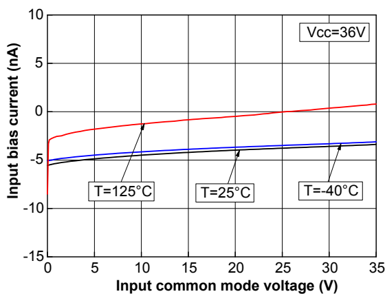
Figure 12. Input bias current vs common mode voltage at V_{CC} = 36\text{ V}
