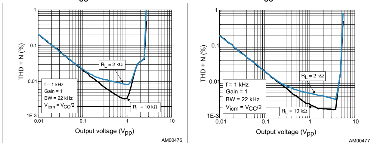
Figure 18. THD+N vs. output voltage at V_{CC} = 2.7\text{ V} Figure 19. THD+N vs. output voltage at V_{CC} = 5.5\text{ V}
