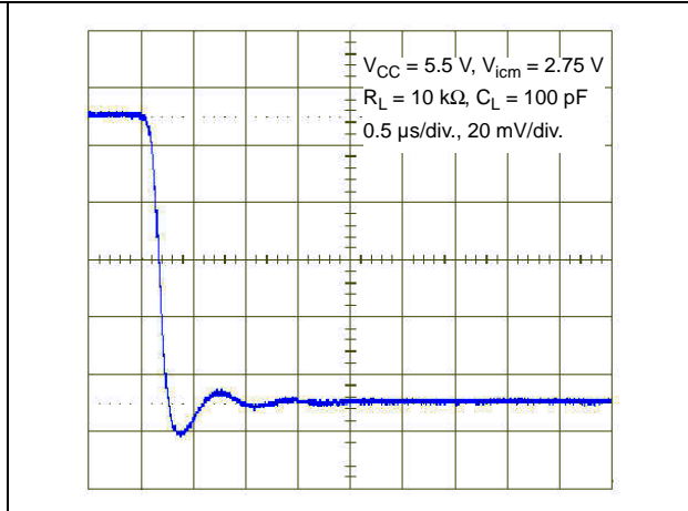
Figure 22. Response to a 100 mV input step for gain = 1 at V_{CC} = 5.5 V falling edge
