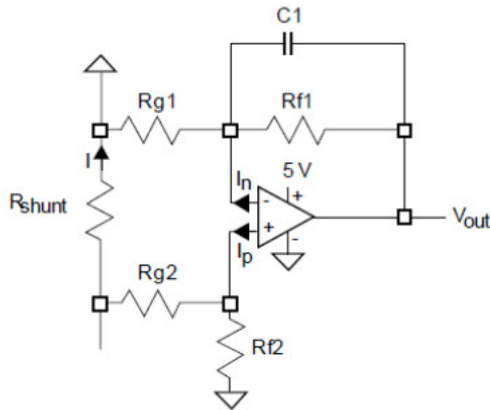
Figure 48. Low-side current sensing schematic
