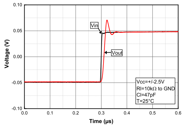
Figure 28. Small step response at V_{CC} = 5 V
