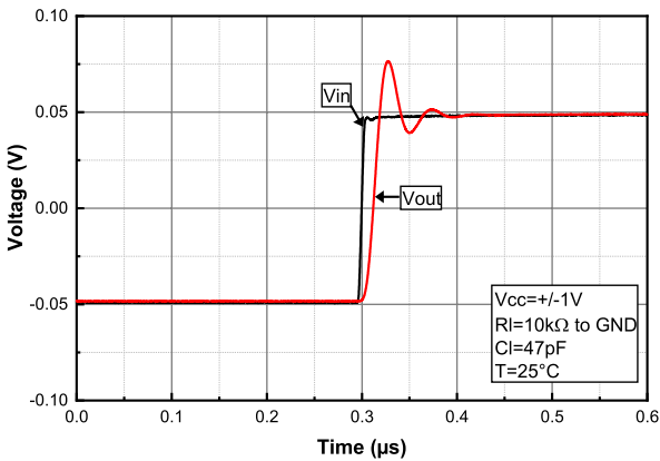
Figure 29. Small step response at V_{CC} = 2 V
