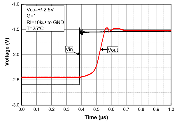
Figure 30. Desaturation from low rail at V_{CC} = 5 V
