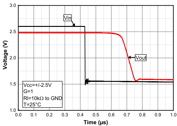
Figure 31. Desaturation from high rail at V_{CC} = 5 V
