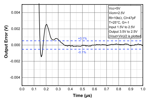
Figure 32. Settling time output high to low at V_{CC} = 5 V
