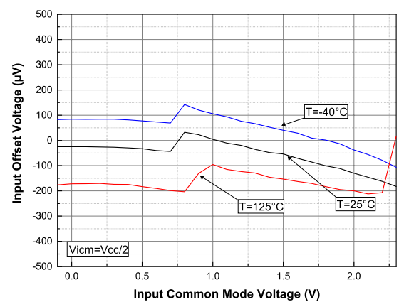
Figure 12. Input offset voltage vs. common mode voltage at V_{CC} = 2.2\text{ V}
