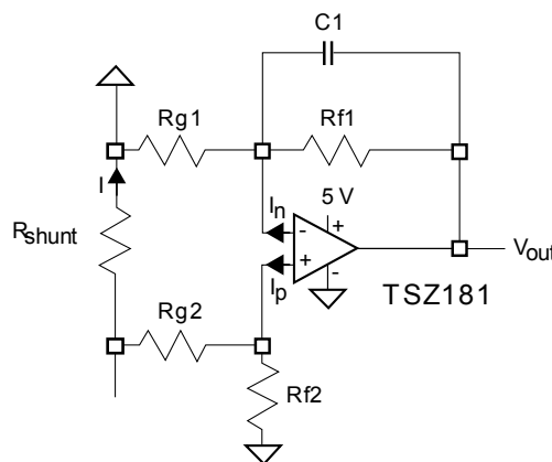
Figure 64. Low-side current sensing schematic
