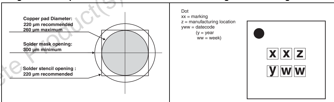
Figure 17. Footprint recommendations
