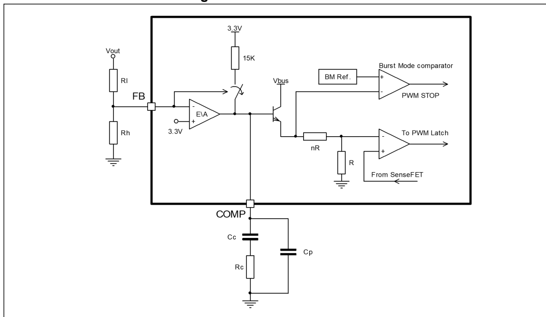
Figure 21. Feedback circuit
