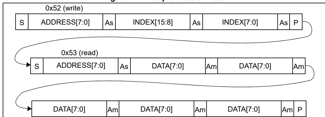
Figure 27. Multiple location read
