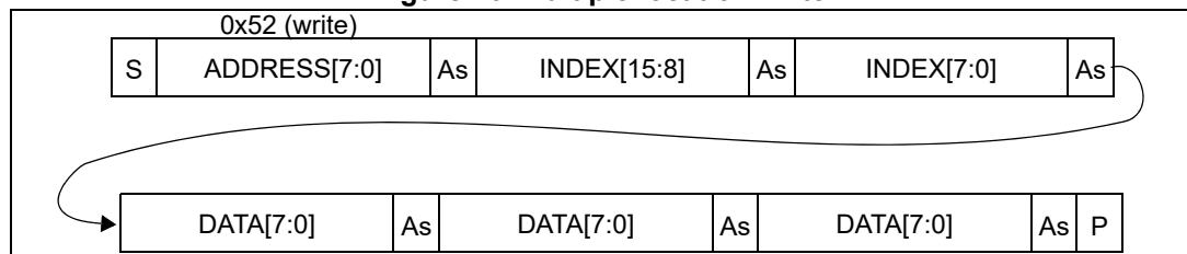
Figure 26. Multiple location write
