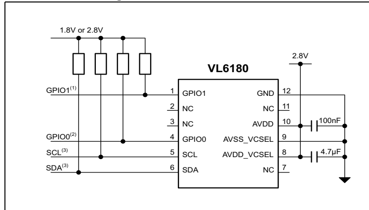
Figure 3. VL6180 schematic
