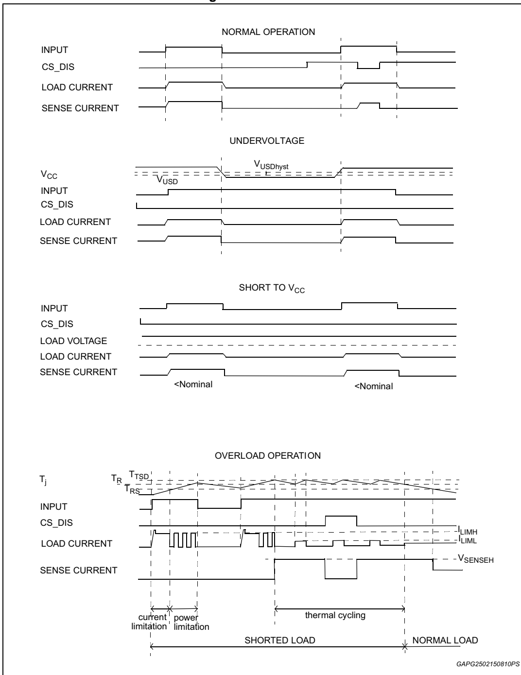
Figure 35. Waveforms
