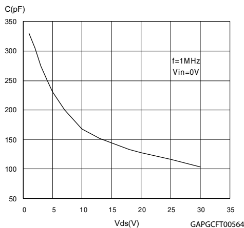
Figure 23. Capacitance variations
