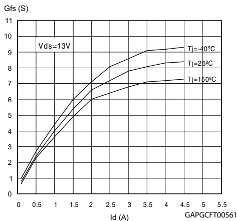
Figure 20. Transconductance
