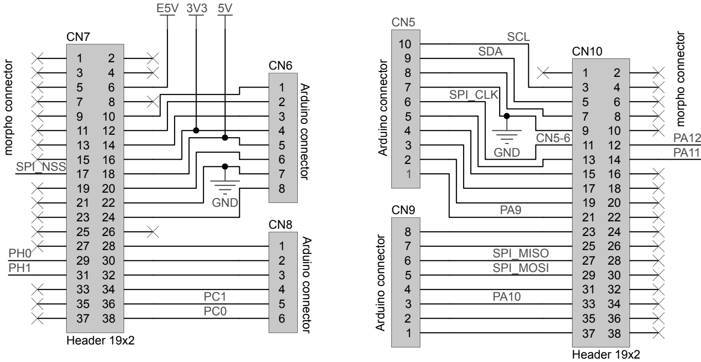
Figure 2. X-NUCLEO-SAFEA1 circuit schematic - Arduino and morpho connectors
