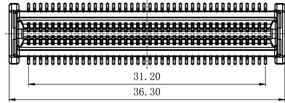
80PIN: BB41-80FT-1B-XHR
