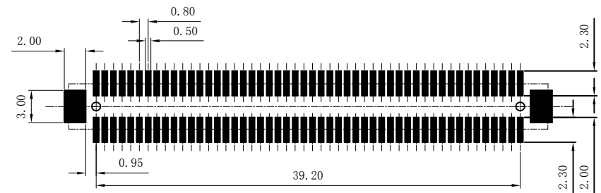
RECOMMENDED PCB LAYOUT TOLERANCE: ±0.05mm
