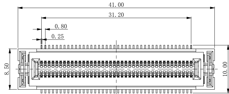
80PIN: BB42-80AT-1B-XHR
