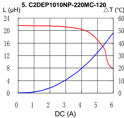
Temperature Chart
