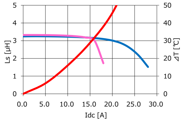
CDEP15D90T150NP-6R2MC-125
