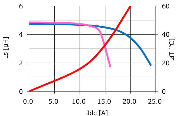
CDEP15D90T150NP-4R7MC-125
