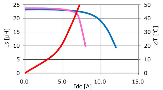
CDEP15D90T150NP-220MC-100
