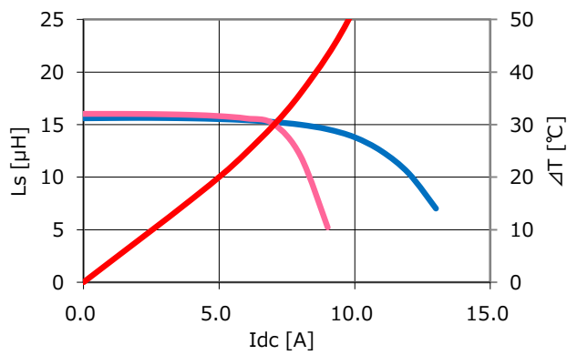
CDEP15D90T150NP-150MC-125
