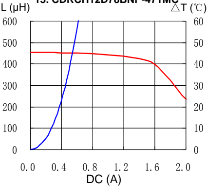
13. CDRCH12D78BNP-471MC
