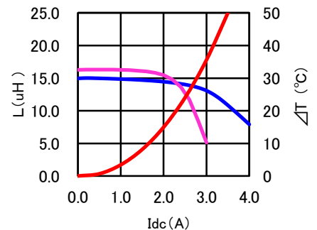
CDRH80D65BT150NP-150MC
