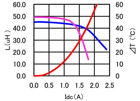
CDRH80D65BT150NP-151MC
