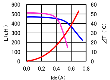
CDRH80D65BT150NP-471MC
