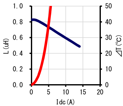
CY0420AT125DS-R82MC
