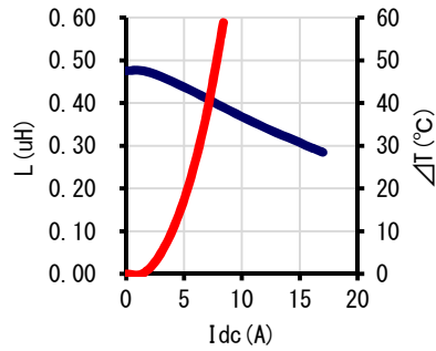
CY0420AT125DS-R47MC
