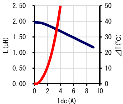
CY0420AT125DS-2R2MC
