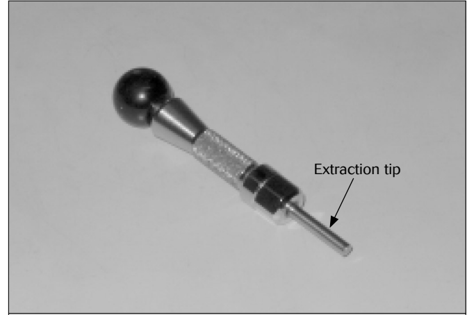
Extraction tooling 5106.021.09.24
