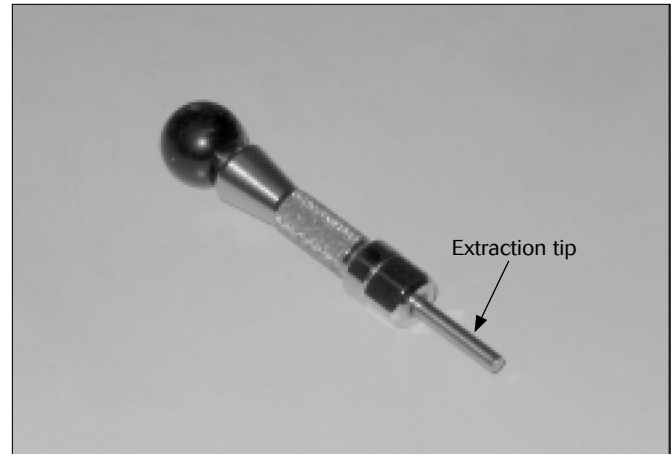
Extraction tooling 5106.021.09.36
