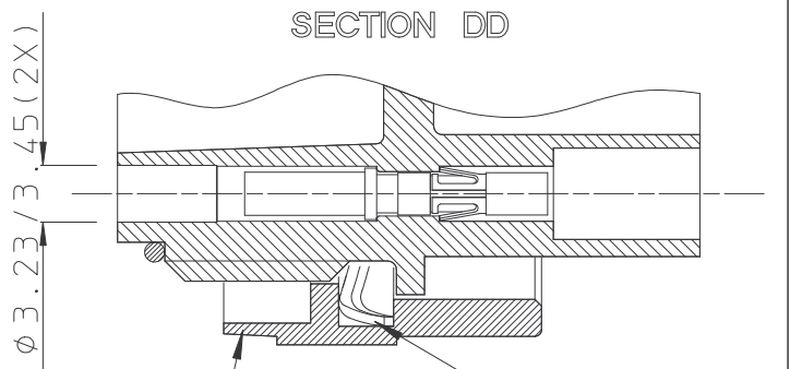
FEMALE POWER CONTACTS (7*): SEE NOTE 1
